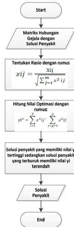
Gambar 6. Penelusuran MOORA
