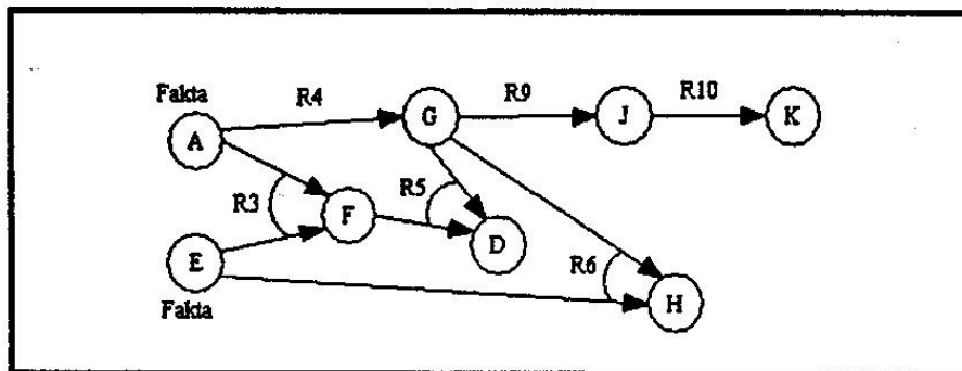
Gambar 1. Metode Forward Chaining
